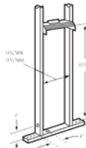
Rough-In Dimensions
