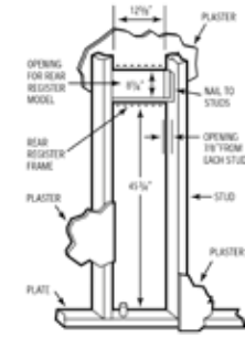
Rear Register Rough-In
