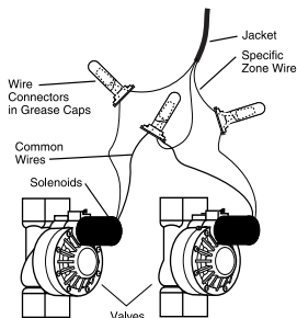
Figure 19: Wiring Valves
