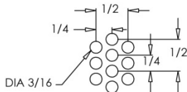
Perforated Screen Detail
