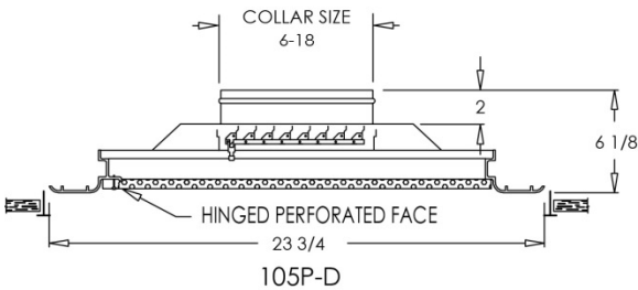
Shown with Optional Square Collar
