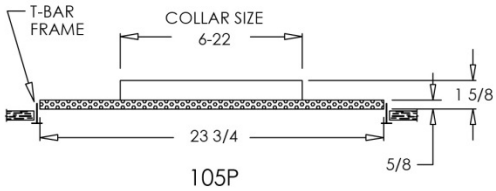
Shown with Optional Square Collar
