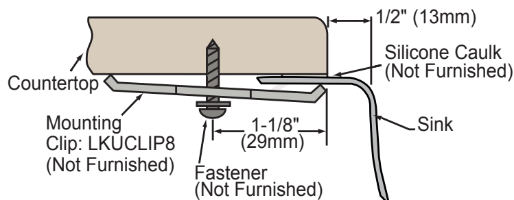
Installation Profile 1/2"(13mm) Reveal
