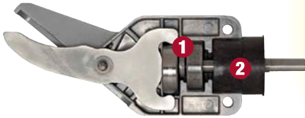
1. Long-life, dual ball bearings 2. Non-slip flats on drive shaft.
