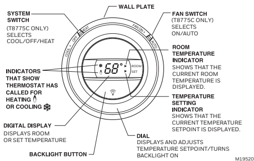
Fig. 10. T8775 Thermostat (features and operation).
