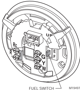
Fig. 7. Fuel switch.
