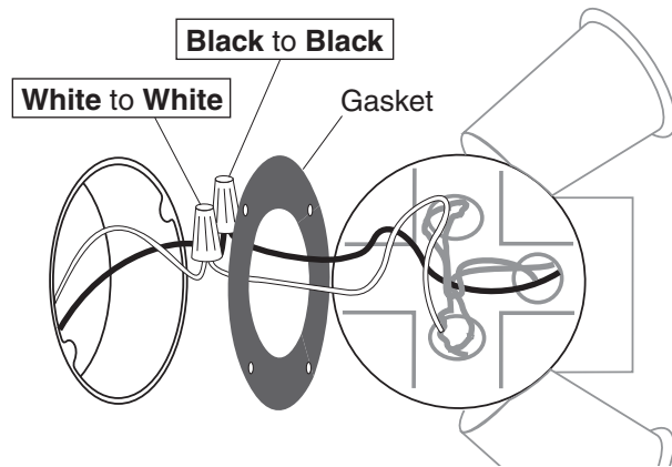
Wall Mount
