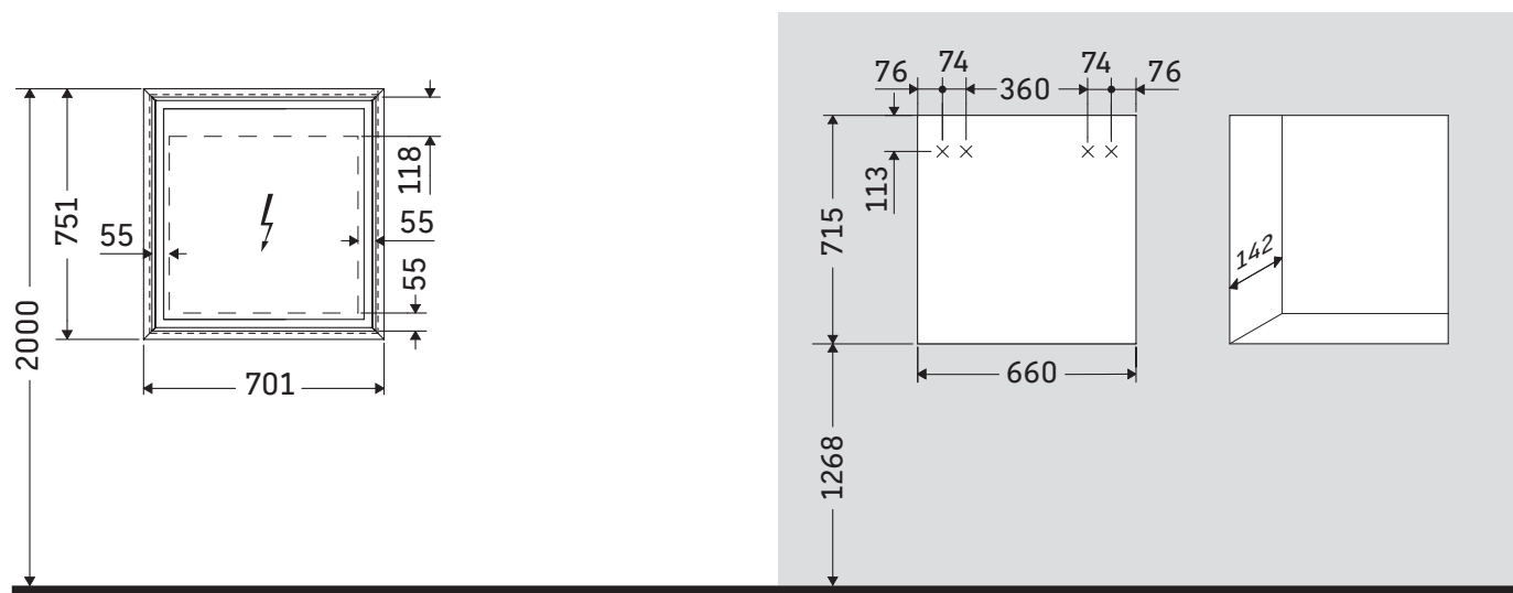
Cutout dimensions for built-in cabinets
