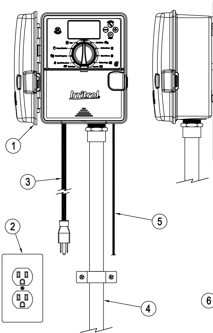
INDOOR INSTALLATION
