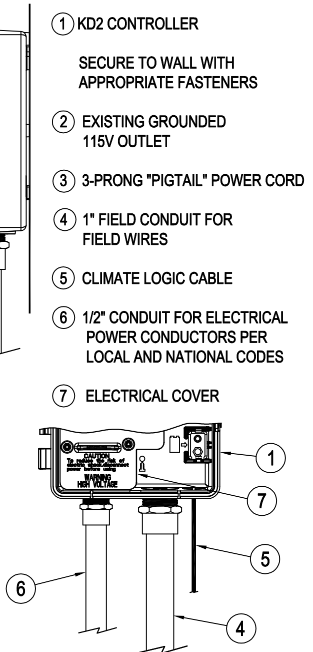
OUTDOOR INSTALLATION
