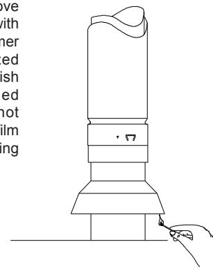
FIG. 15 MATCH TEST FOR SPILLAGE
