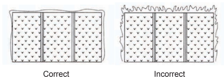
FIGURE 5 Correct Burner Flame Pattern
