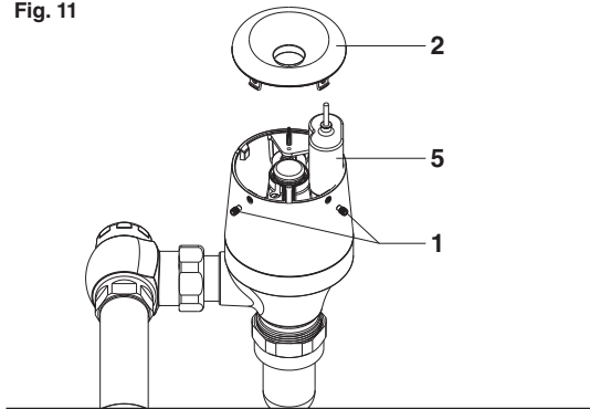
Fig. 11a STANDARD BATTERY
