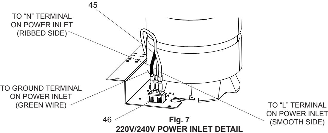
220V/240V POWER INLET DETAIL
