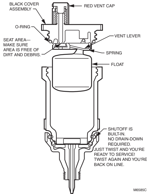
EA122A construction
