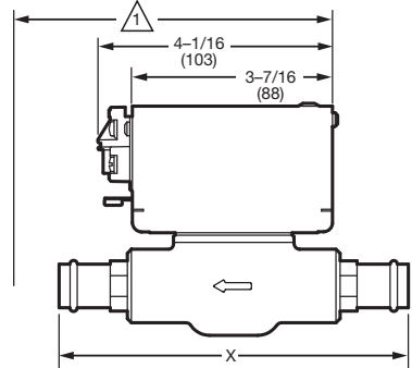
Dimensions (V8043F). Measurements in inches (mm). See Table below.
