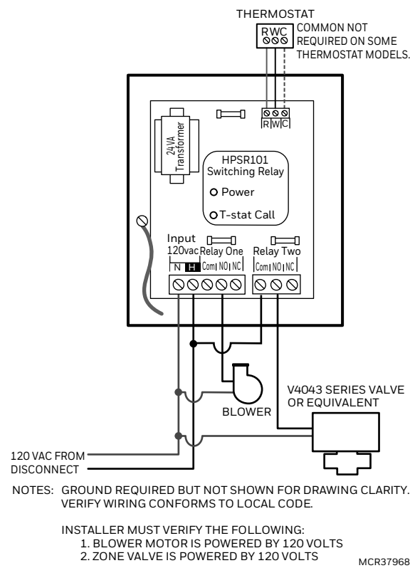
HPSR101 Switching Relay with 120 volt valve and blower fan.
