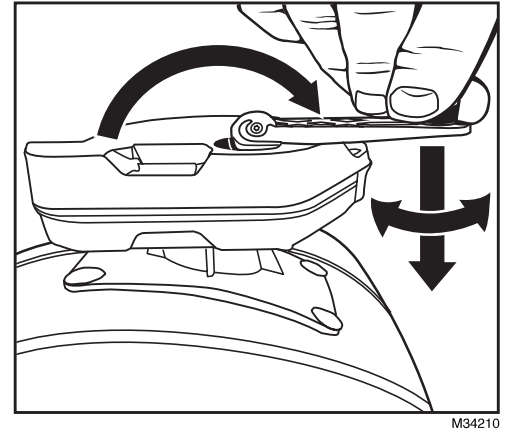
Fig. 4. Adjustment crank.
