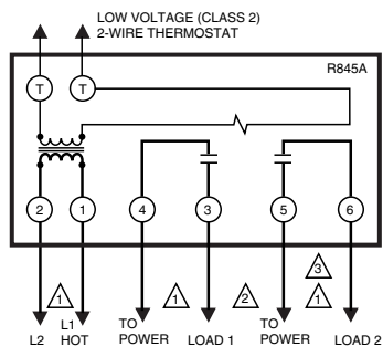
Fig. 8—R845A hookup for controlling two loads.
