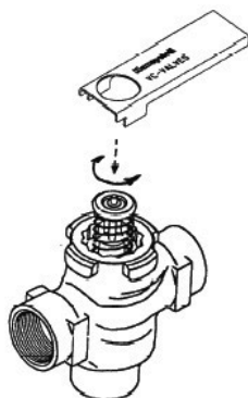
Fig. 5. Installing Cartridge
