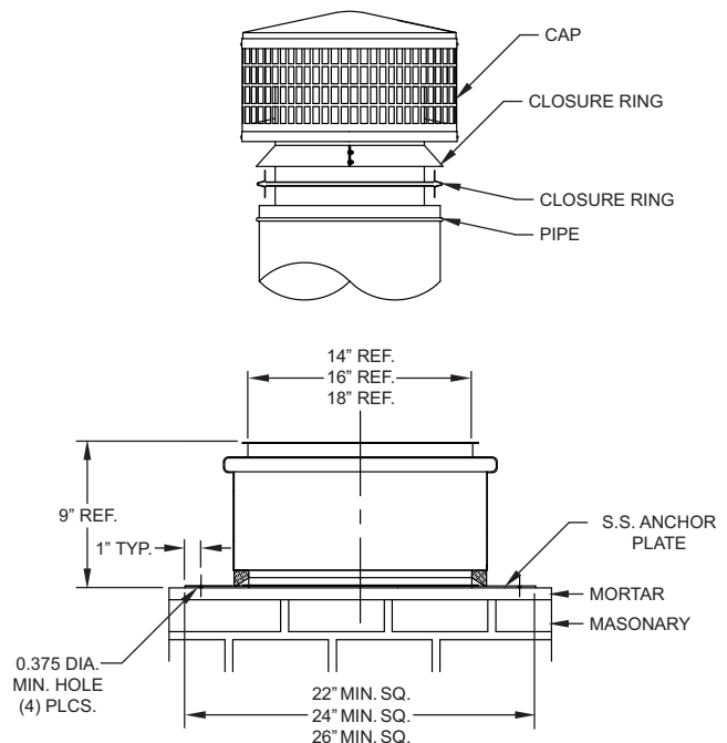
FIG. 15b 14TG, 16TG, AND 18TG ANCHOR PLATE
