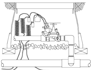
Brass Electric Remote Control EFB-CP Valve
