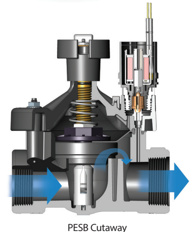
PESB Cutaway
