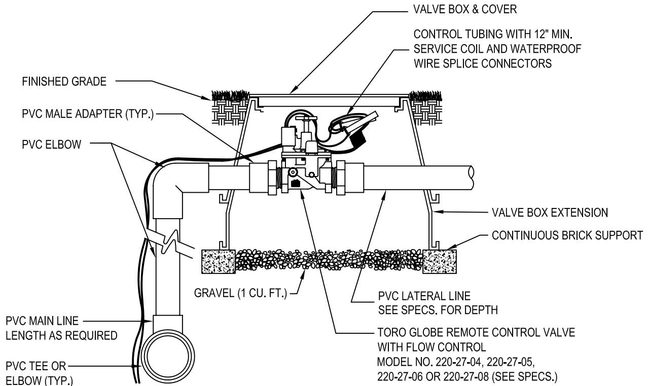
SECTION/ELEVATION NOT TO SCALE
